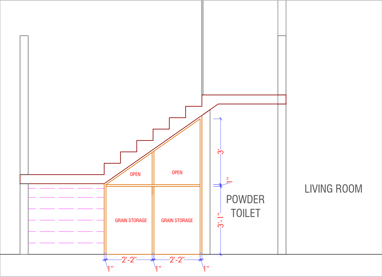
SECTION AA'
