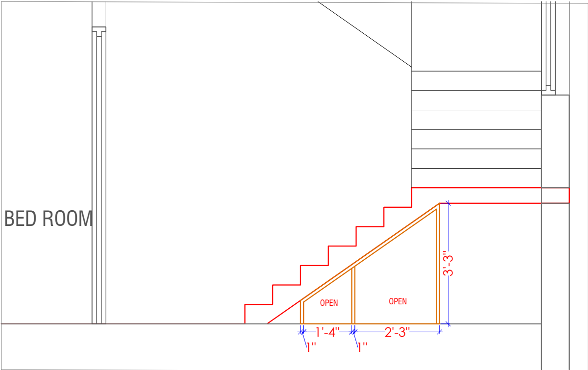
ELEVATION C
