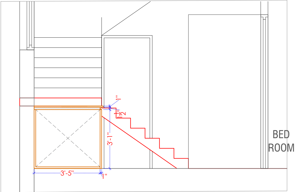
SECTION BB'
